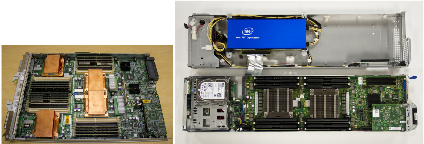
Figure 1.15: Left: a four-socket design. Right: a two-socket design with co-processor.
