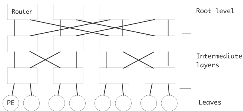
Figure 2.27: A fat-tree built from simple switching elements
