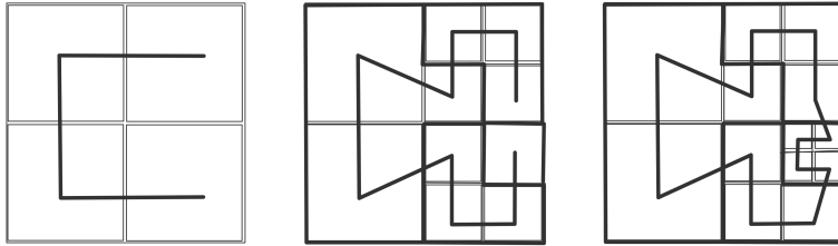
Figure 2.36: Space filling curves, regularly and irregularly refined
