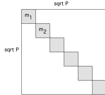
Figure 10.4: IMP realization of the 1.5D N-body problem
