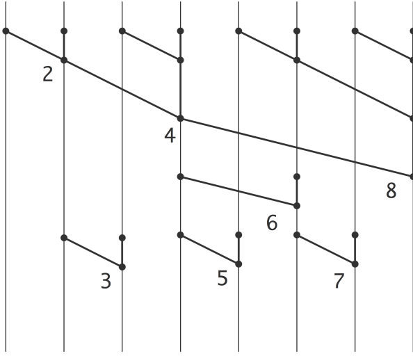
Figure 19.1: A prefix operation applied to 8 elements
