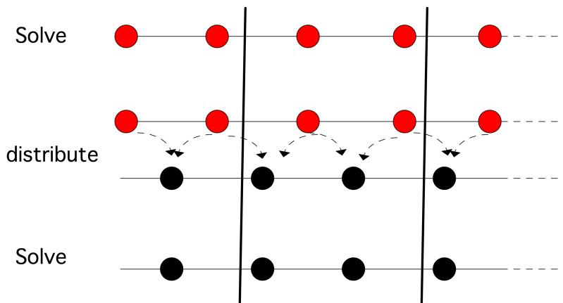
Figure 6.21: Parallel red-black solution on a 1d domain
