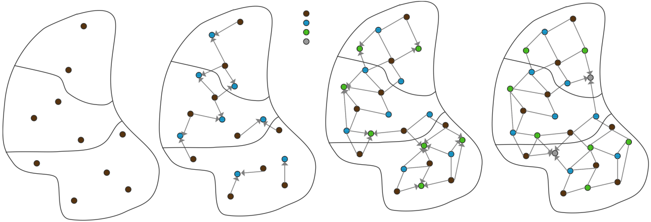
Figure 6.24: Solving a parallel multicolour ILU in four steps
