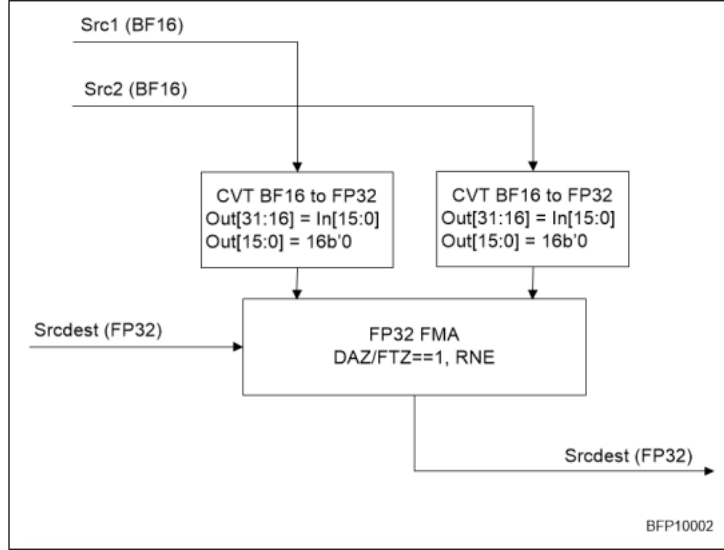
Figure 3.4: An FMA unit taking two bfloat16 and one fp32 number. (illustration from [34])
