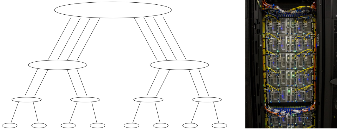
Figure 2.26: A fat tree with a three-level interconnect (left); the leaf switches in a cabinet of the Stampede cluster (right)
