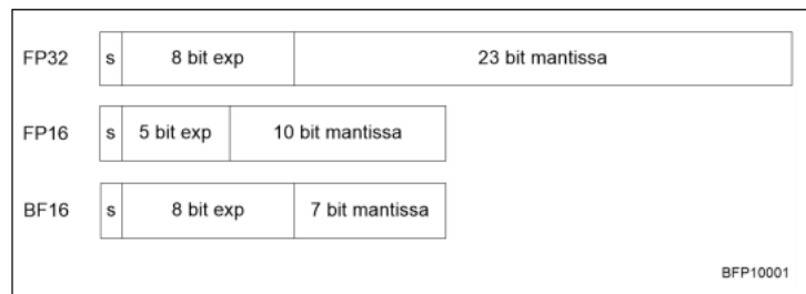
Figure 3.3: Comparison of fp32, fp16, and bfloat16 formats. (Illustration from [34])
