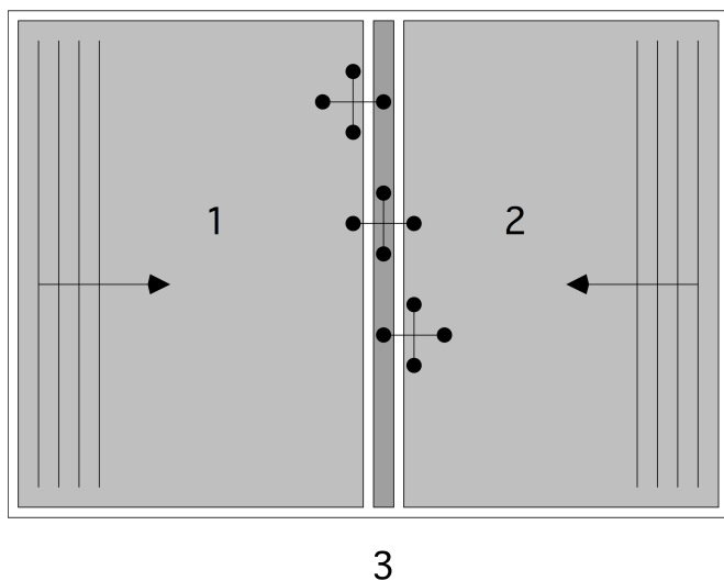
Figure 6.16: Domain dissection into two unconnected subdomains and a separator
