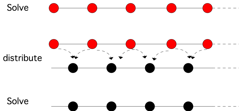
Figure 6.20: Red-black solution on a 1d domain
