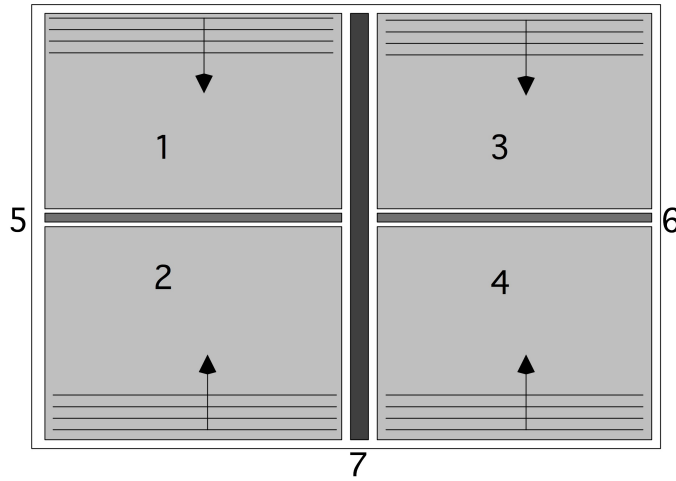
Figure 6.17: A four-way domain decomposition
