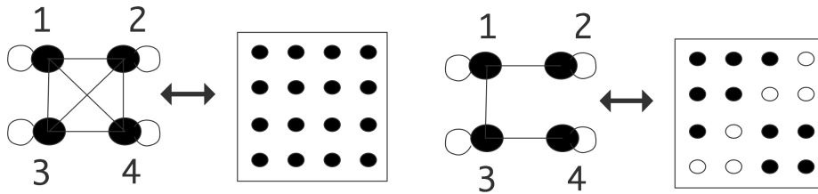
Figure 17.3: A dense and a sparse matrix, both with their adjacency graph
