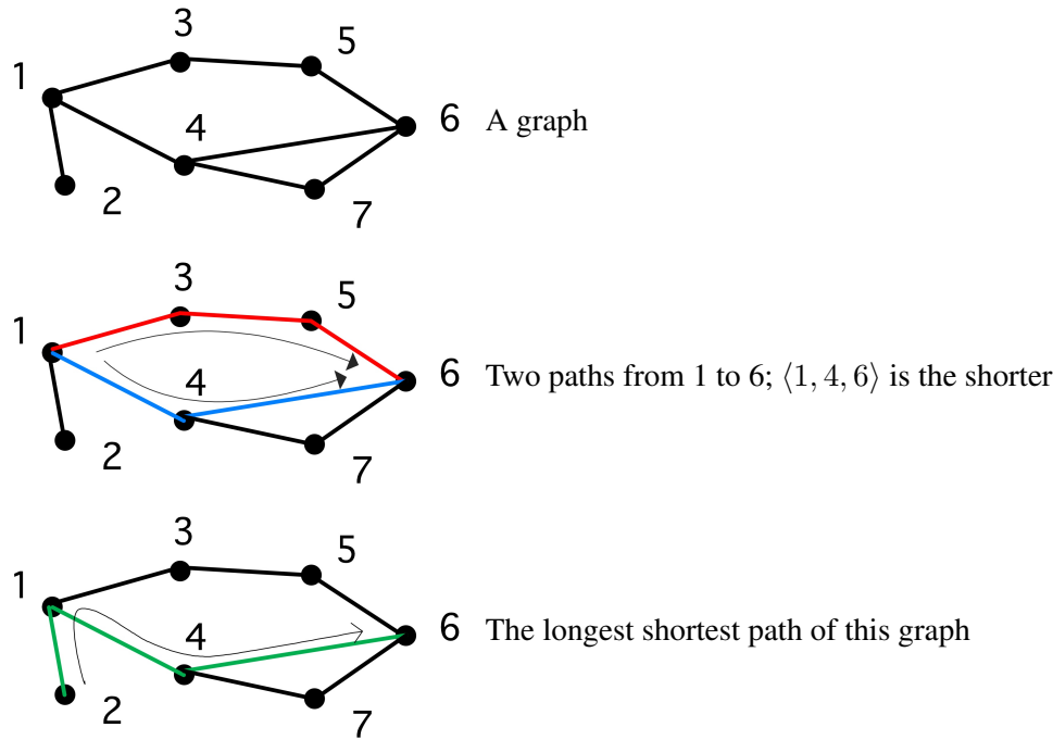
Figure 17.2: Shortest paths
