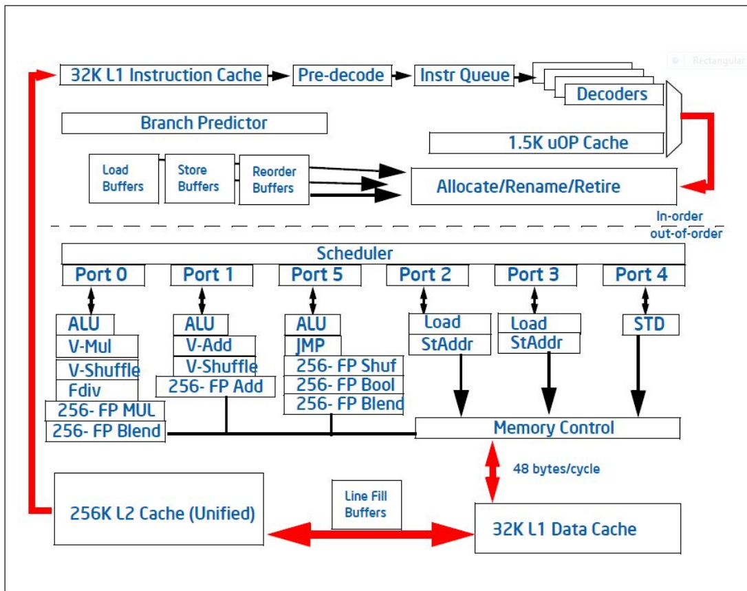
Figure 1.2: Block diagram of the Intel Sandy Bridge core
