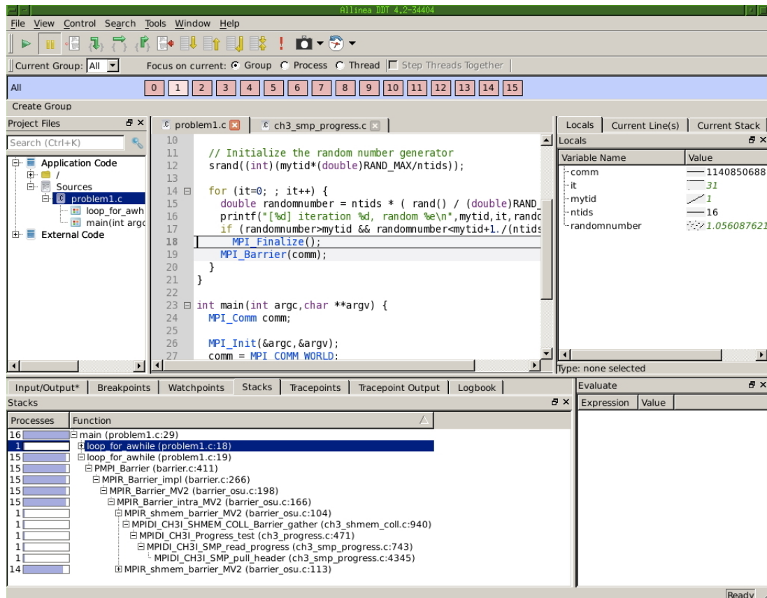
Figure 27.1: Display of 16 processes in the DDT debugger
