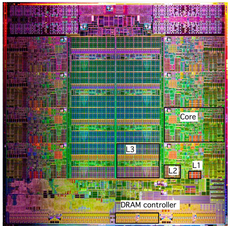
Figure 1.1: The Intel Sandy Bridge processor die
