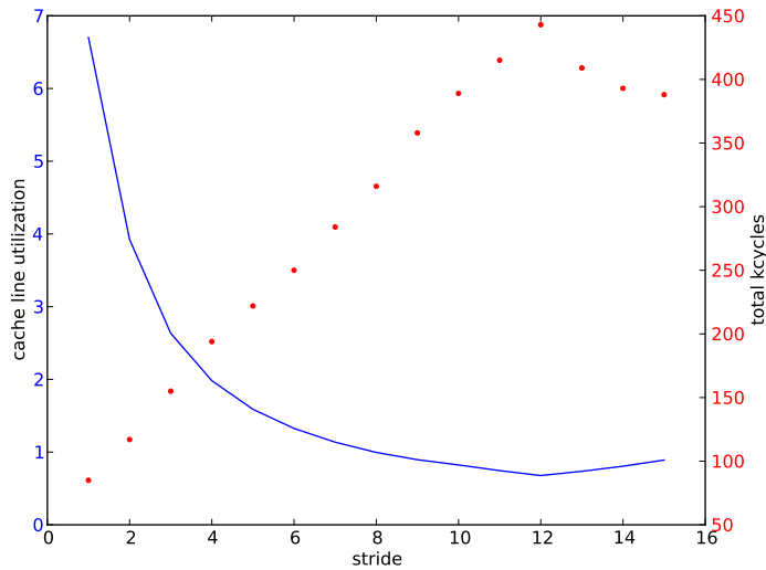
Figure 32.1: Run time in kcycles and L1 reuse as a function of stride
