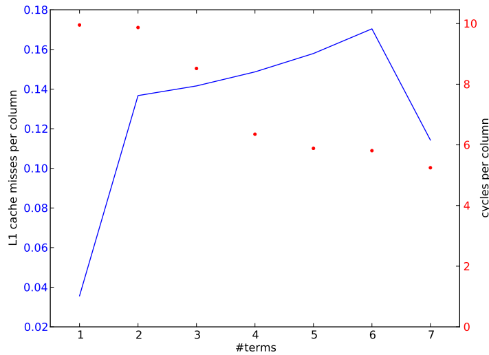
Figure 1.23: The number of L1 cache misses and the number of cycles for each j column accumulation, vector length 4096 + 8
